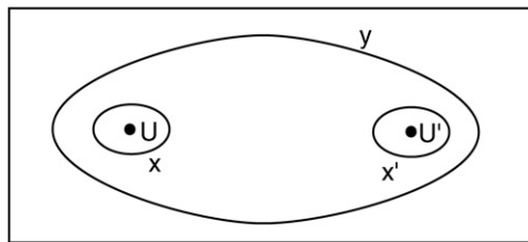
Fig. 1. The 2-punctured disk.
