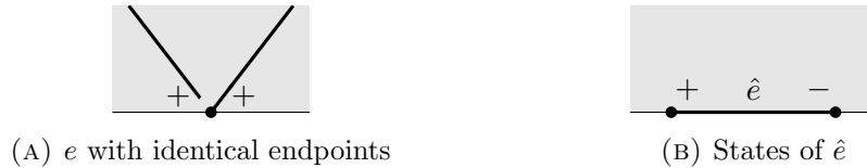
FIGURE 6. Height convention, states of boundary arcs \hat{e}
