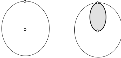
FIGURE 5. Once-punctured monogon \mathcal{M}_1 (left) as the result of attaching an ideal triangle to a bigon (shaded).
