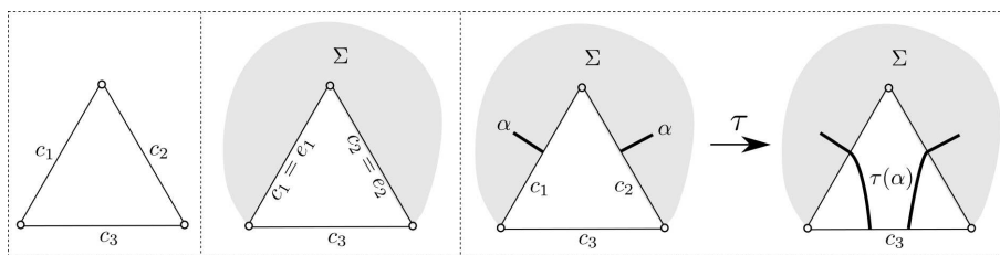
FIGURE 4. Ideal triangle, attaching an ideal triangle to \Sigma , and the map \tau
